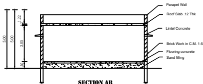
SECTION AB
