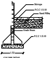
COLUMN DETAIL
