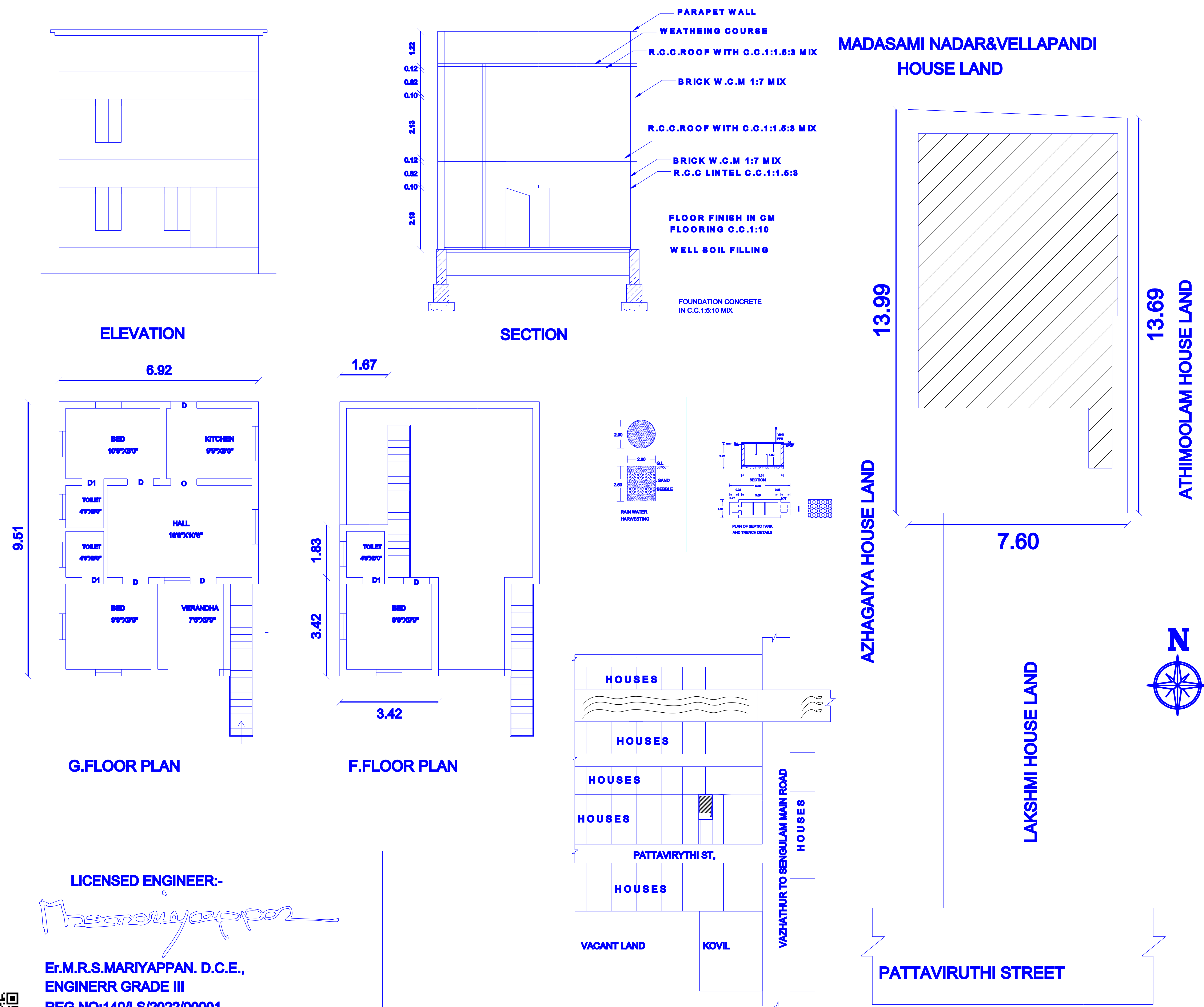
KEY PLAN
