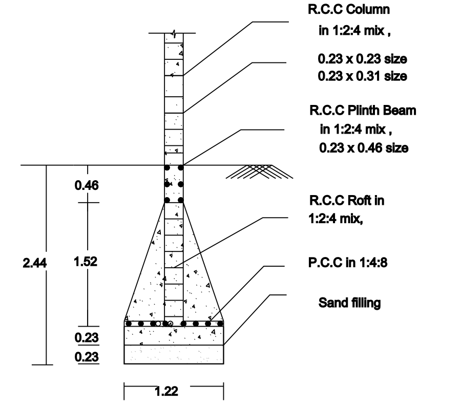
COLUMN DETAILS
