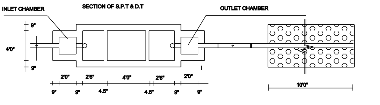
SEPTIC TANK DETAILS
