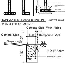
RAIN WATER HARVESTING PIT (1.0M X 1.5M X 1.5M SIZE)
