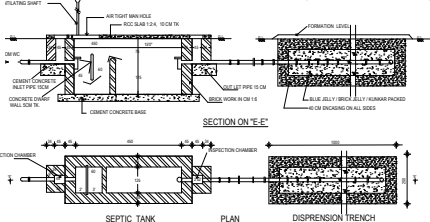
PE DESIGN FOR A SEPTIC TANK 10,000 Lts CAPACITY (NOT TO SCALE)
