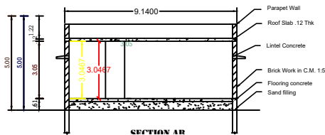
SECTION AB
