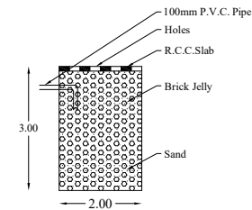
SECTION OF RAIN WATER COLLECTING TANK
