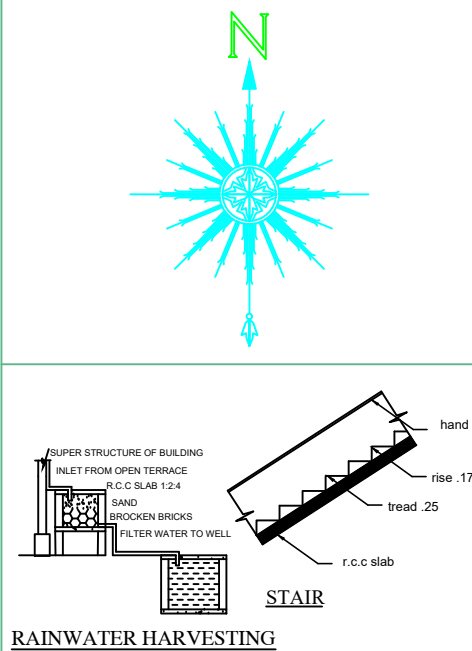
RAINWATER HARVESTING
