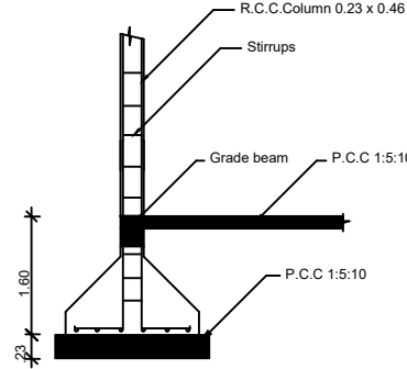
COLUMN DETAIL
