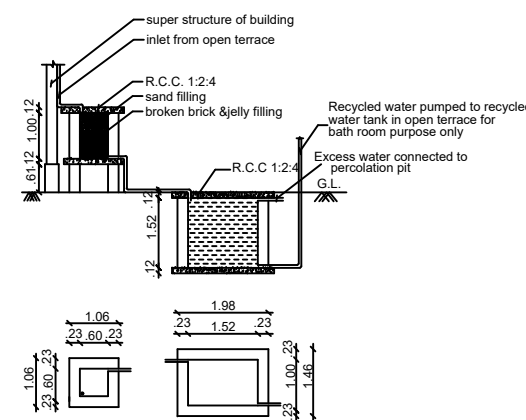
Sump and Filter Bed
