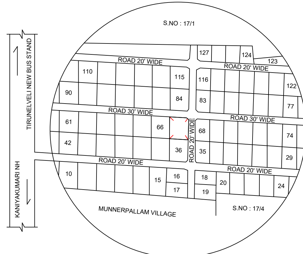
TOPO PLAN ( NOT TO SCALE )
