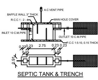
SEPTIC TANK & TRENCH
