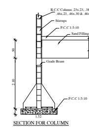
SECTION FOR COLUMN
