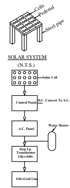
SOLAR SYSTEM FLOW DIAGRAM
