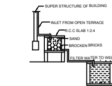
DETAILS OF FILTER BED & WELL
