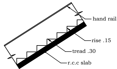
STAIR
