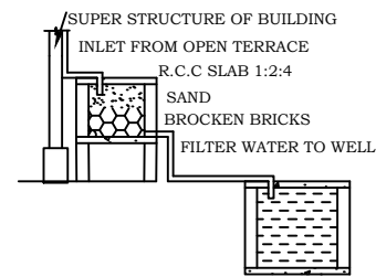
RAINWATER HARVESTING
