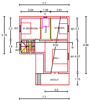
GROND FLOOR PLAN
