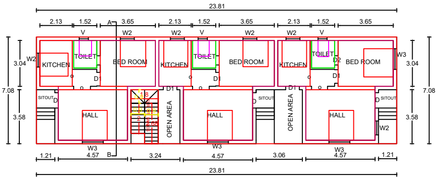
GROND FLOOR PLAN
