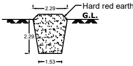
TRIAL PIT (Scale 1:100)
