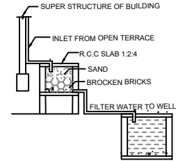
DETAILS OF FILTER BED & WELL
