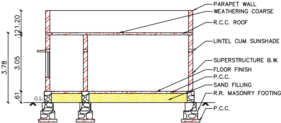
CROSS SECTION ON AA
