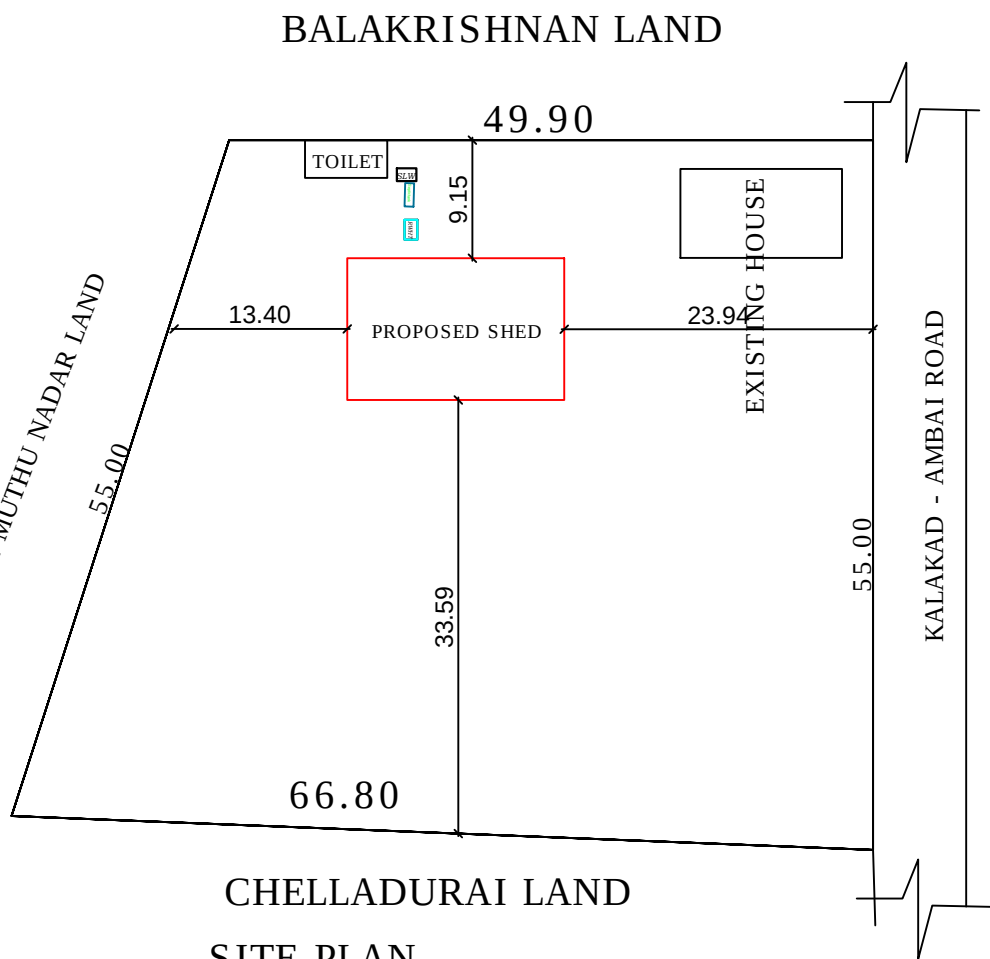
SITE PLAN
