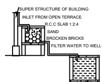
RAINWATER HARVESTING
