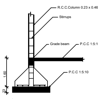
COLUMN DETAIL
