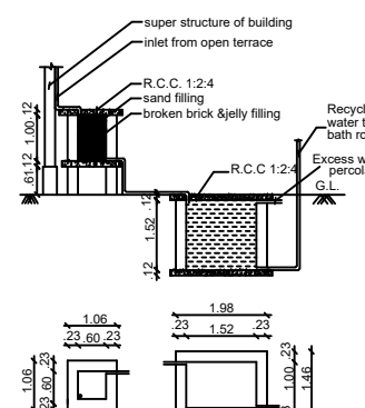
Sump and Filter Bed
