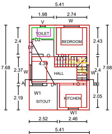
GROND FLOOR PLAN
