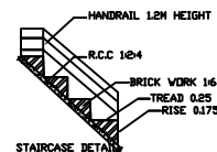
STAIRCASE DETAIL
