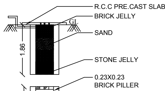
PLAN AND SECTION OF RAINWATER COLLECTION WELL
