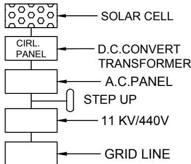
SOLAR SYSTEM FLOW DIAGRAM
