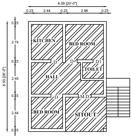
EXG GROUND FLOOR PLAN
