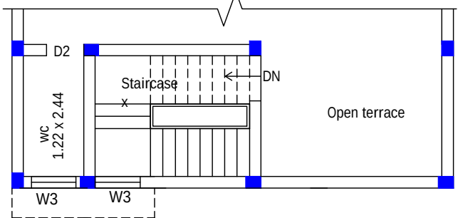
HEAD ROOM PLAN
