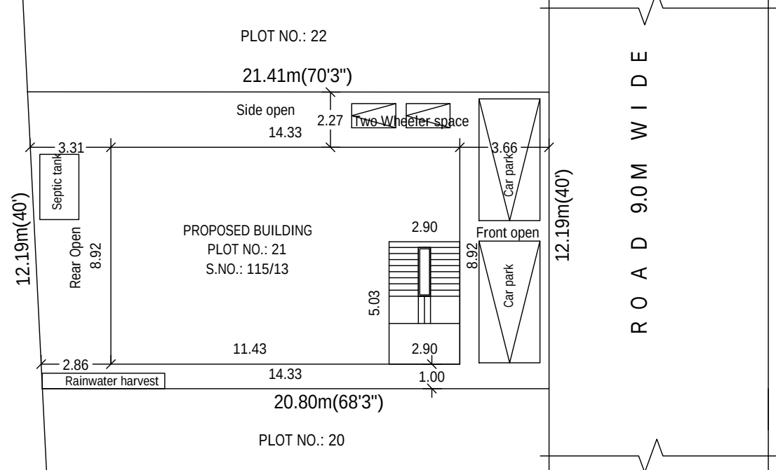
SITE PLAN
