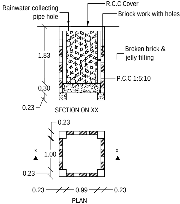
RAINWATER HARVEST WELL
