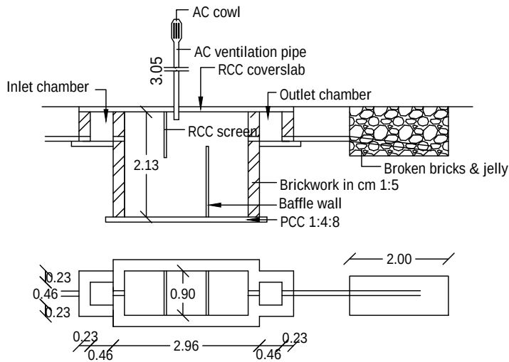
SEPTICTANK DETAILS
