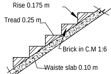
STAIR DETAILS
