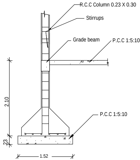
COLUMN DETAIL
