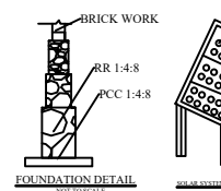
FOUNDATION DETAIL
