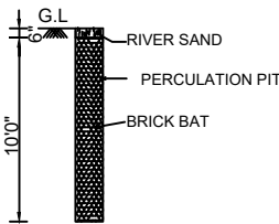
PERCOLATION PIT
