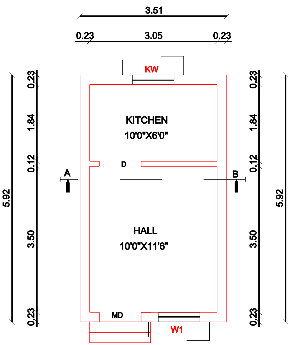
ROUND FLOOR PLAN
