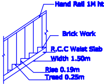
STAIRCASE DETAIL
