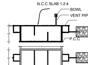
SEPTIC TANK AND TRENCH NTS
