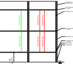
SECTION ON AA
