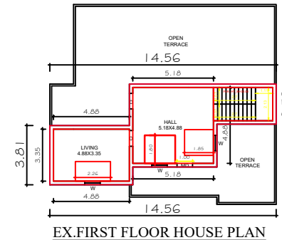
EX.FIRST FLOOR HOUSE PLAN
