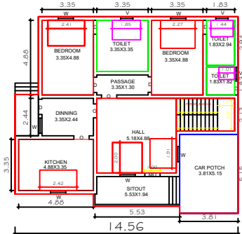
EX.GROUND FLOOR HOUSE PLAN
