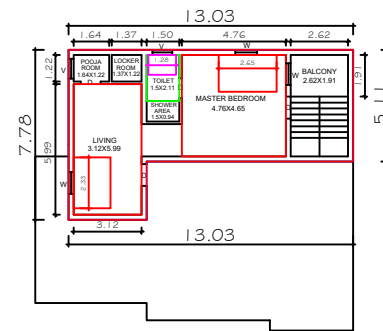
PRO.FIRST FLOOR HOUSE PLAN
