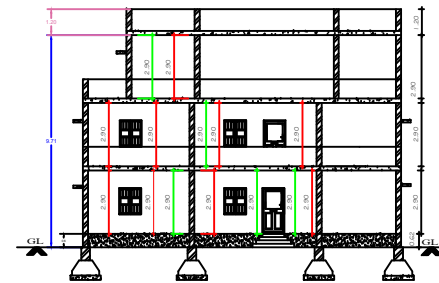
SECTION 1 - A A
