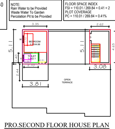
PRO.SECOND FLOOR HOUSE PLAN
