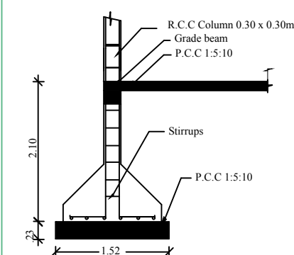
Column Detail
