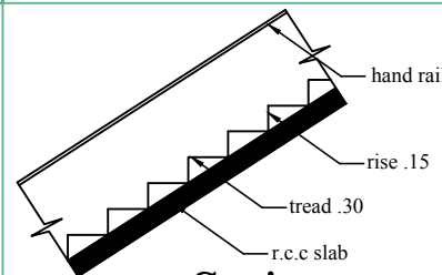
Stair
