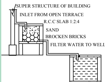
Rainwater harvesting
