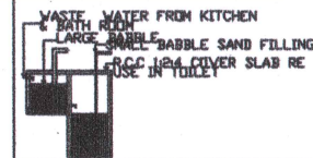
RECYCLING OF WASTE WATER FROM KITCHEN & BATHROOM
