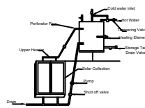
Details Of Solar Water Heater (NTS)
