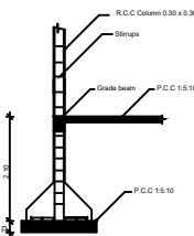
COLUMN DETAIL
