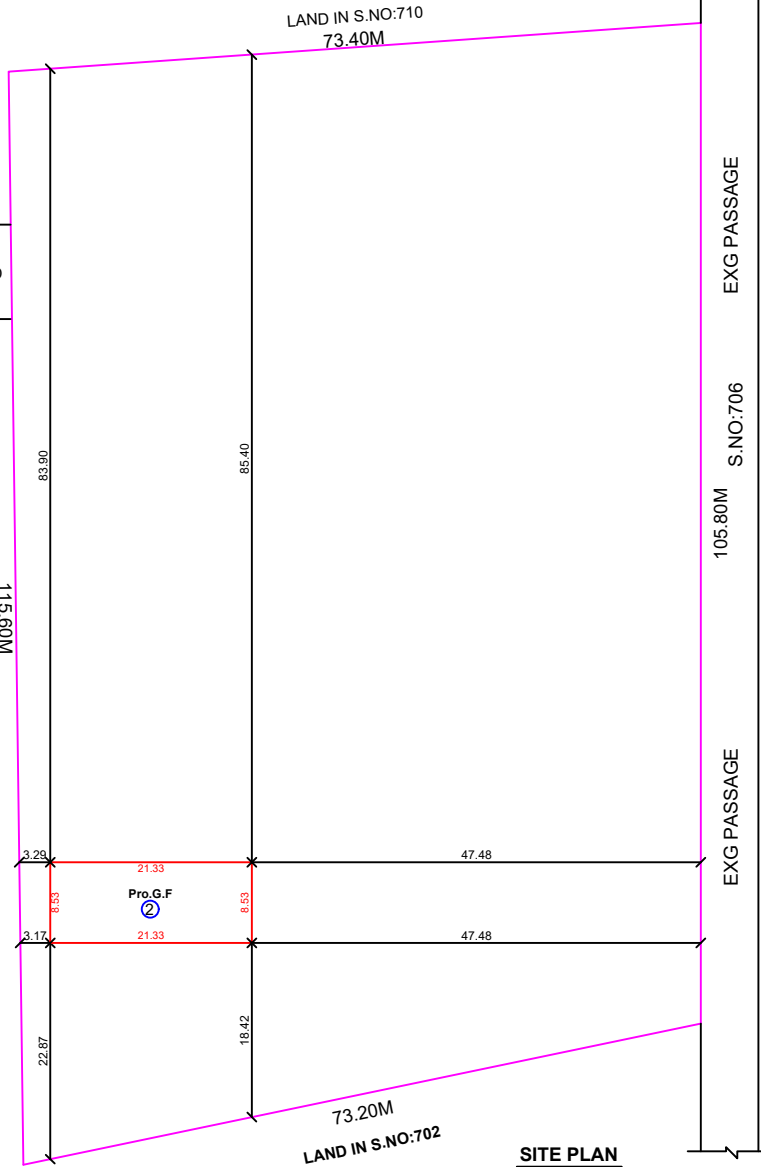
SITE PLAN (SCALE:1:400)
