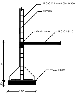
COLUMN DETAIL
