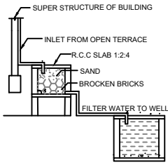
DETAILS OF FILTER BED & WELL NTS
