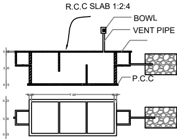
SEPTIC TANK AND TRENCH NTS
