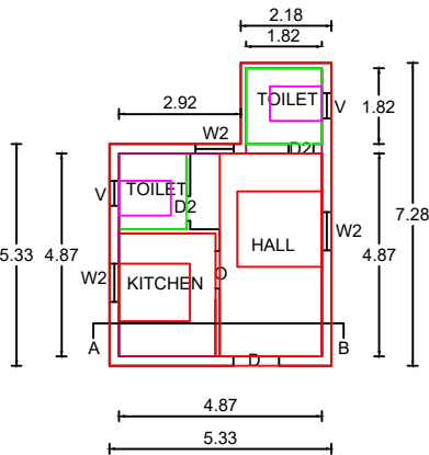
GROND FLOOR PLAN
