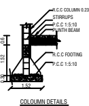
COLUMN DETAILS
