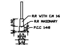
FOUNDATION
