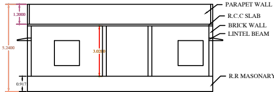
SECTION AT X-X'
