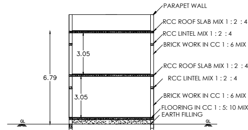
SECTION ON AB & ( HALF ELEVATION)
