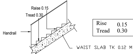
STAIRCASE DETAIL
