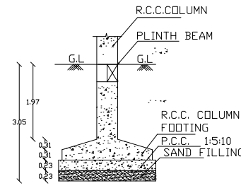
FOUNDATION DETAIL
