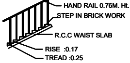
STAIR CASE DETAIL
