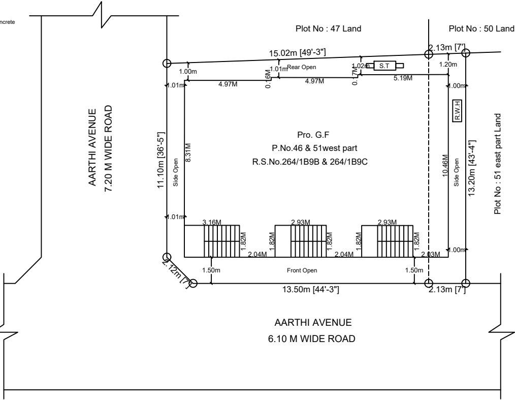
SITE PLAN
