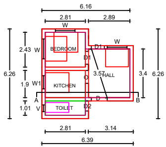
GROND FLOOR PLAN
