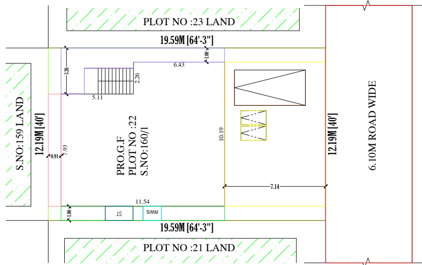
SITE PLAN (1:100)
