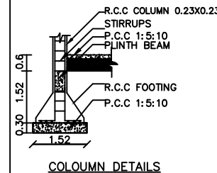
COLOUMN DETAILS
