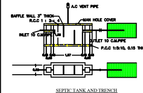
Septic Tank
