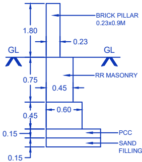
FOOTING DETAILS
