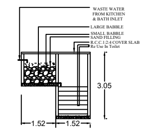
RECYCLING OF WASTE WATER FROM KITCHEN & BATHROOM
