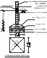
FOUNDATION DETAIL
