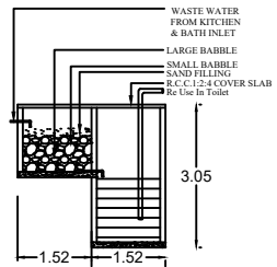
RECYCLING OF WASTE WATER FROM KITCHEN & BATHROOM
