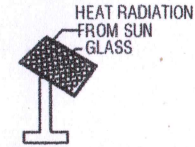
SOLAR SYSTEM
