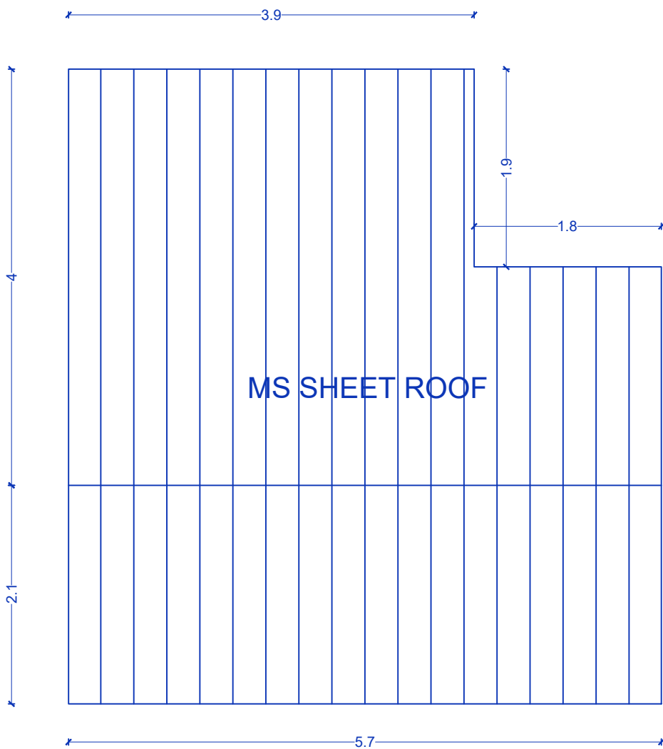
ROOF PLAN
