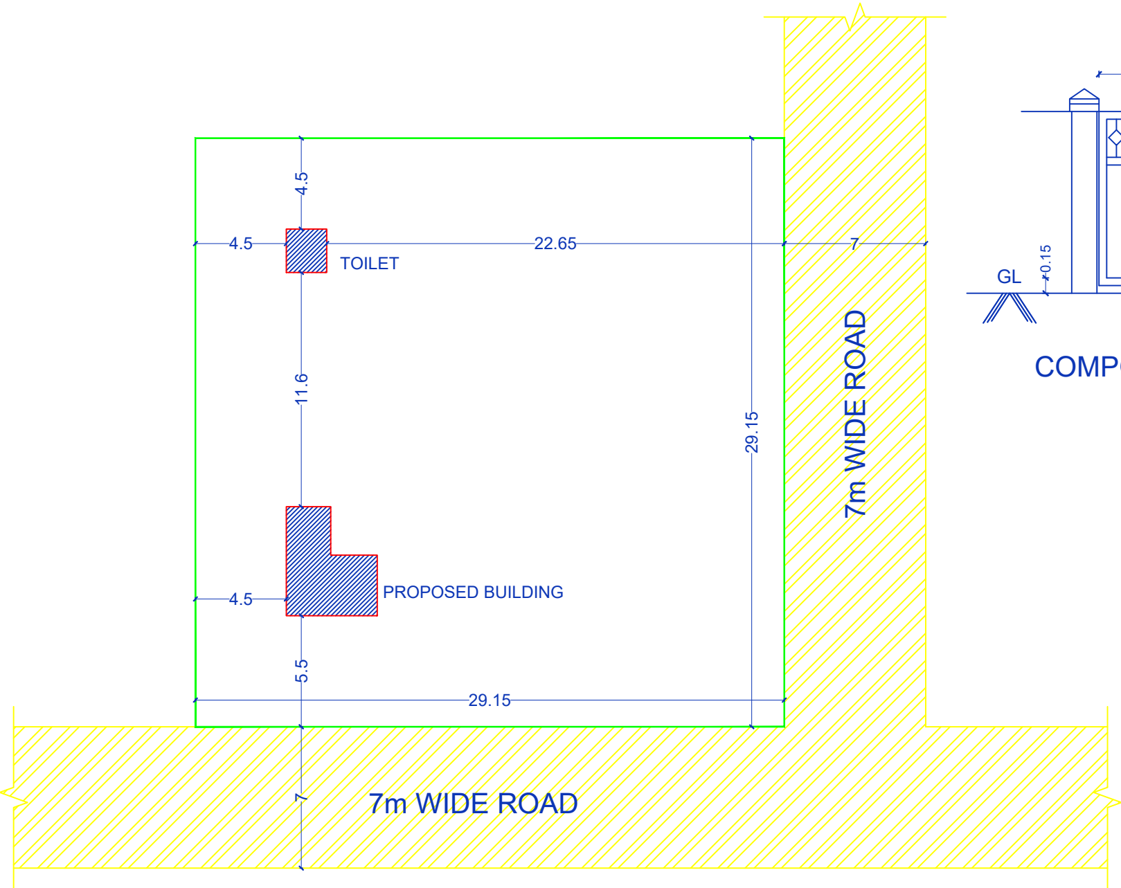
SITE PLAN
