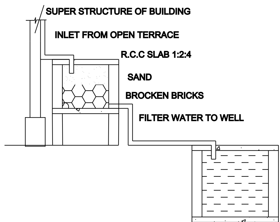
Rainwater harvesting
