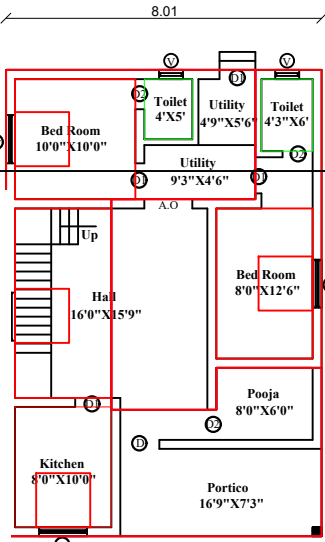
GROUND FLOOR PLAN (Existing & Additional Proposed)
