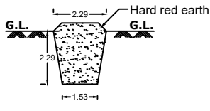
TRIAL PIT (Scale 1:100)
