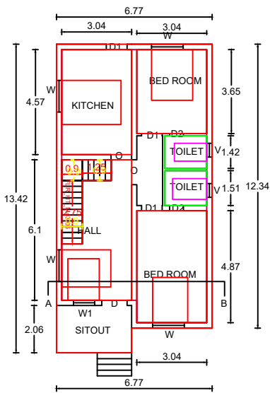
GROND FLOOR PLAN
