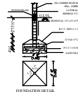
FOUNDATION DETAILS
