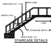
STAIRCASE DETAILS
